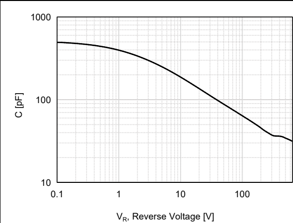
Figure 7. Capacitance Characteristic
