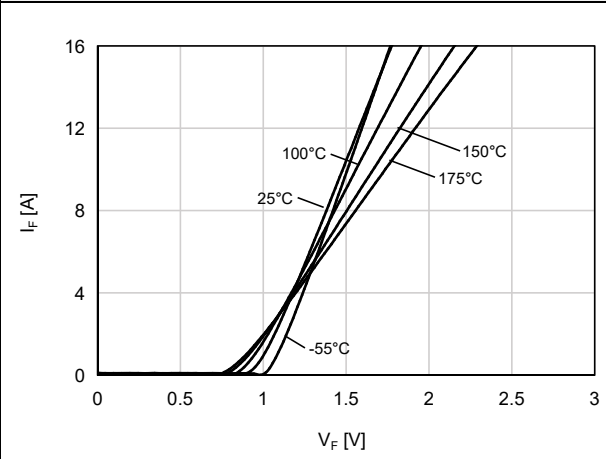
Figure 3. Forward Characteristics
