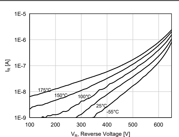
Figure 4. Reverse Characteristics
