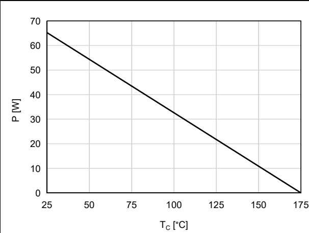
Figure 1. Power Derating
